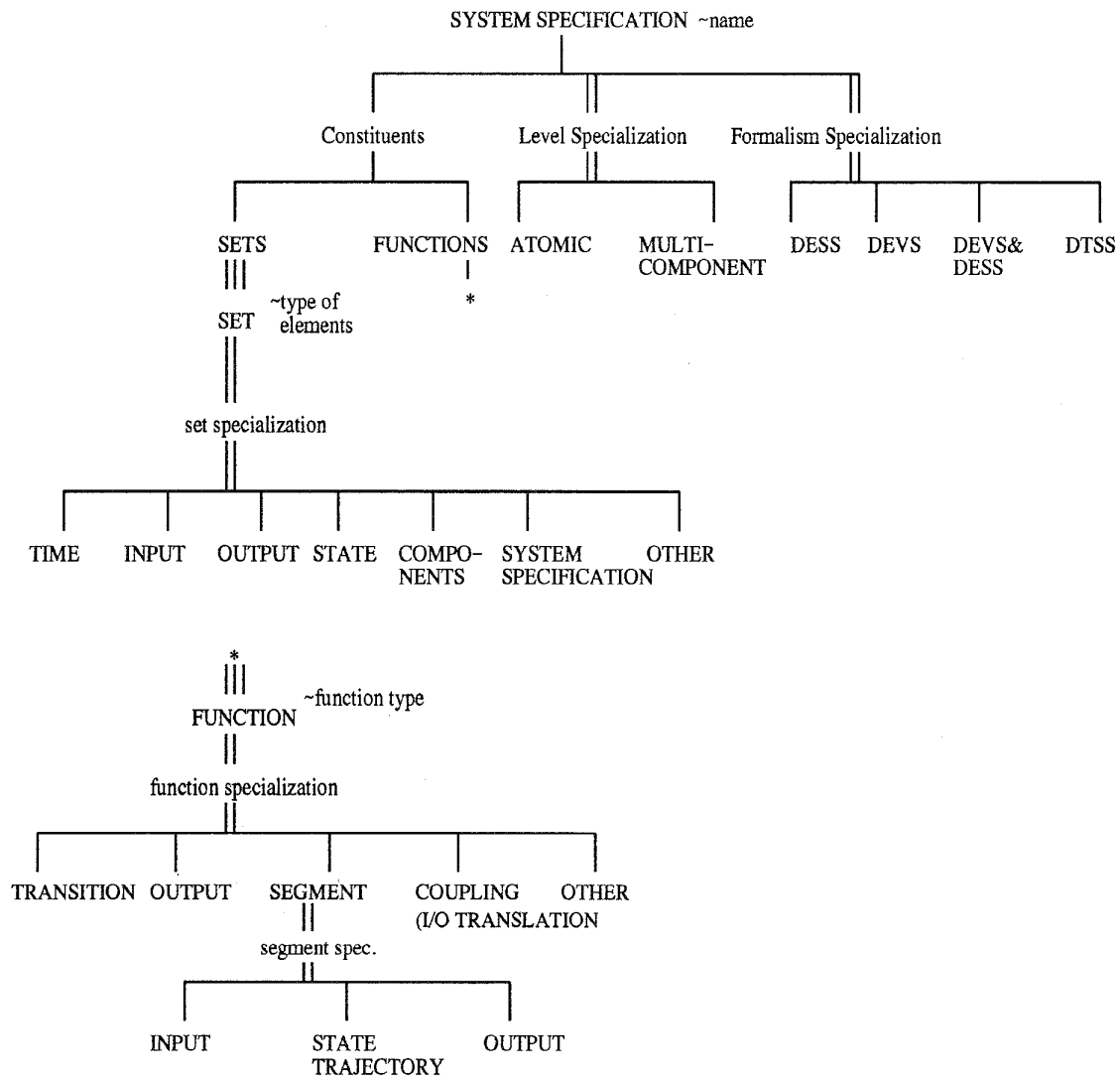
Figure 1: Canonical SES of System Specification Elements
